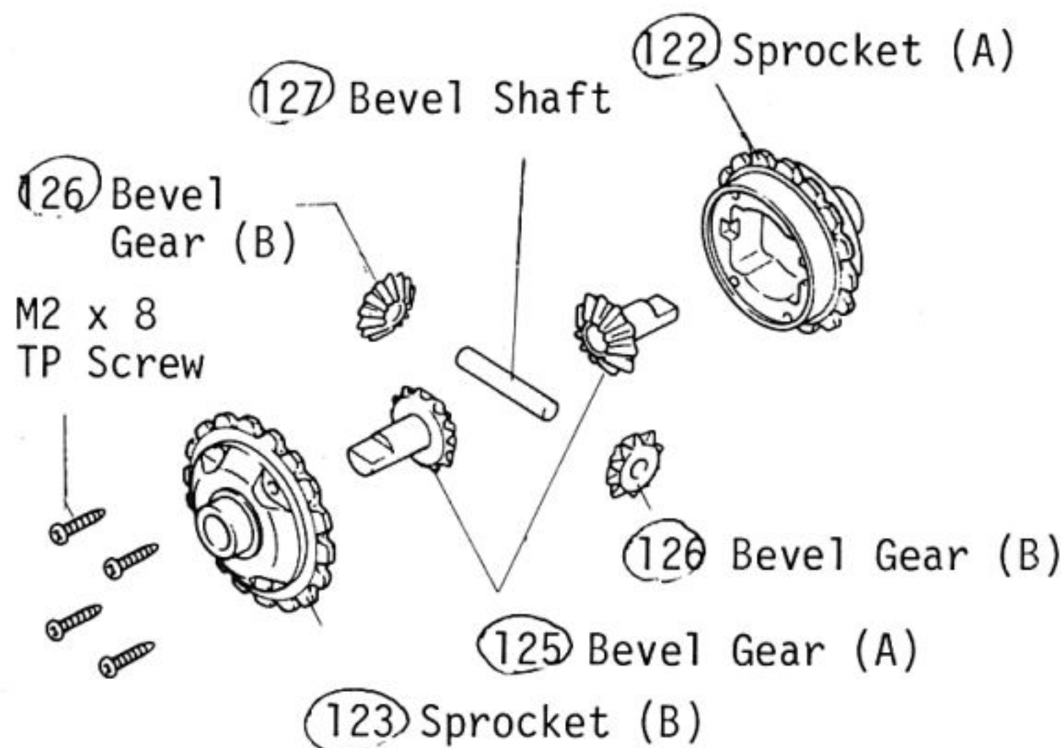
[Front Differential]
